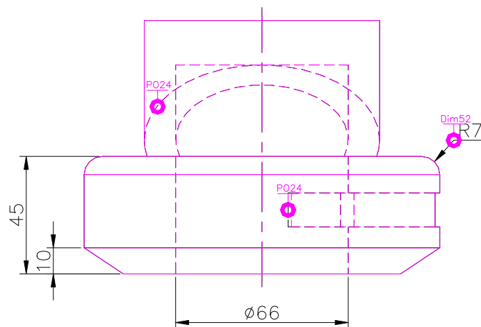
FRONT SCALE 1/2
