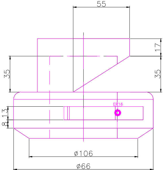
RIGHT SCALE 1/2
