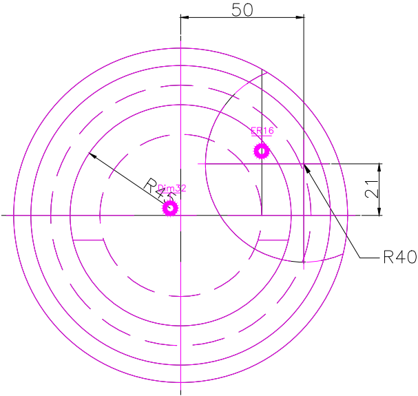
TOP SCALE 1/2
