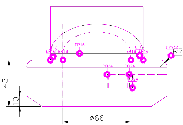
FRONT SCALE 1/2
