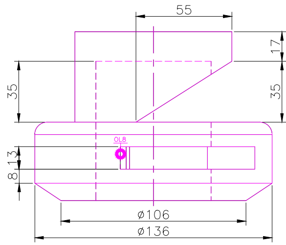
RIGHT SCALE 1/2
