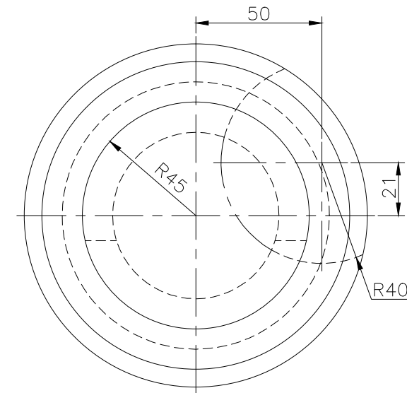
TOP SCALE 1/2
