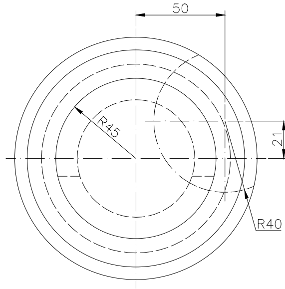
TOP SCALE 1/2
