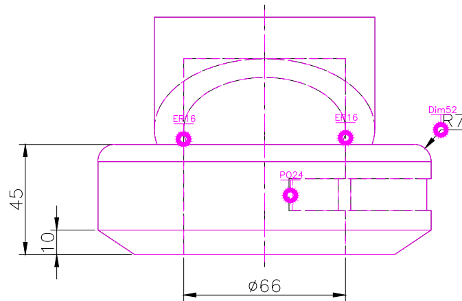
FRONT SCALE 1/2
