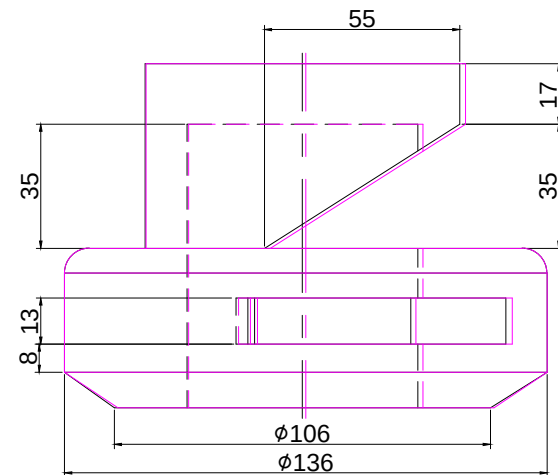
RIGHT SCALE 1/2
