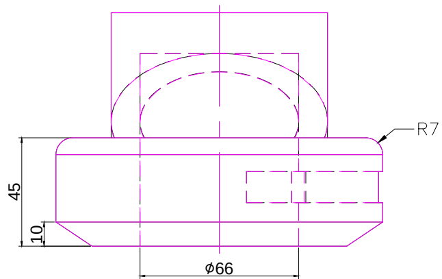
FRONT SCALE 1/2
