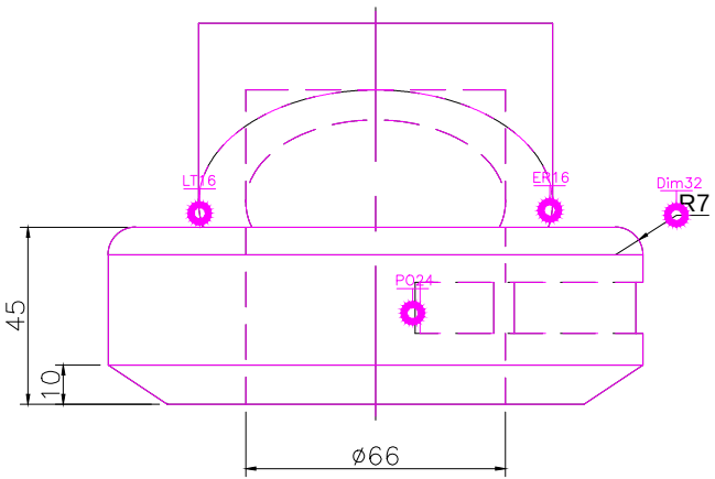
FRONT SCALE 1/2
