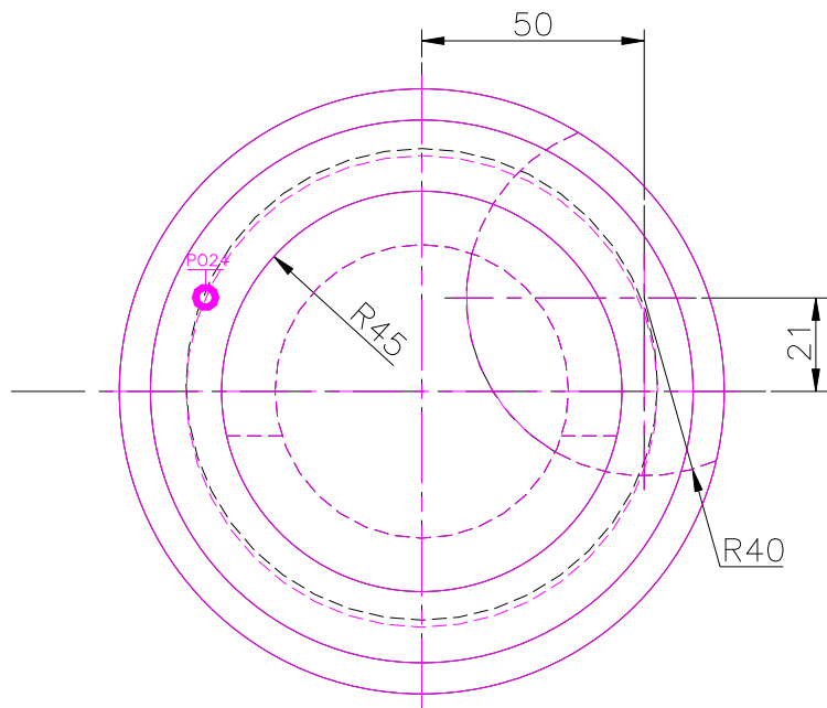
TOP SCALE 1/2
