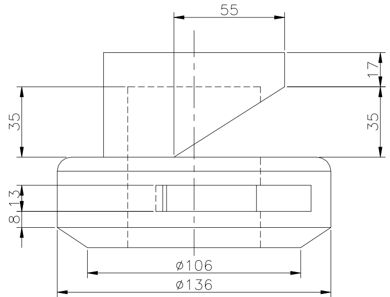
RIGHT SCALE 1/2
