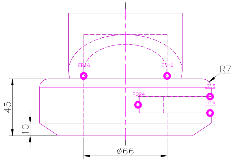
FRONT SCALE 1/2
