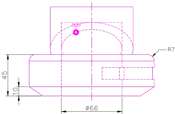
FRONT SACLE 1/2
