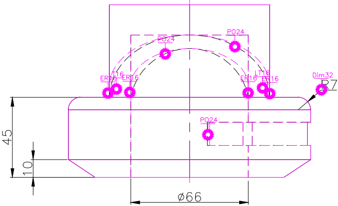
FRONT SCALE 1/2
