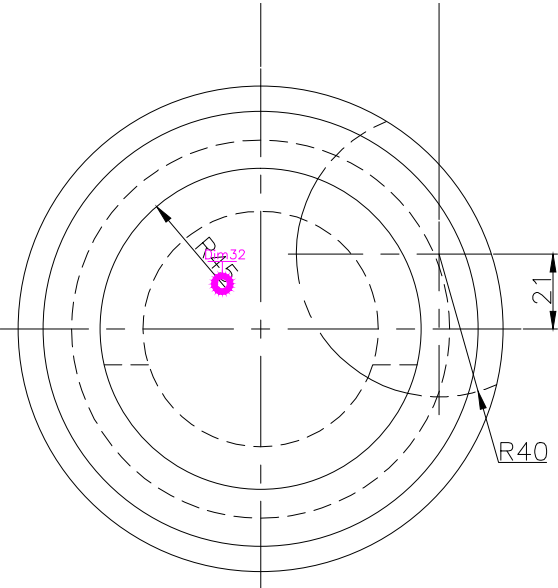
TOP SCALE 1/2
