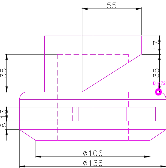
RIGHT SCALE 1/2
