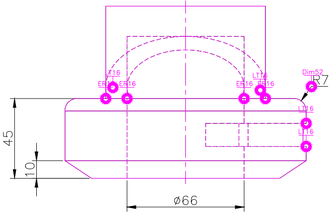
FRONT SCALE 1/2
