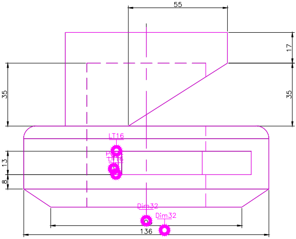
RIGHT SCALE 1/2
