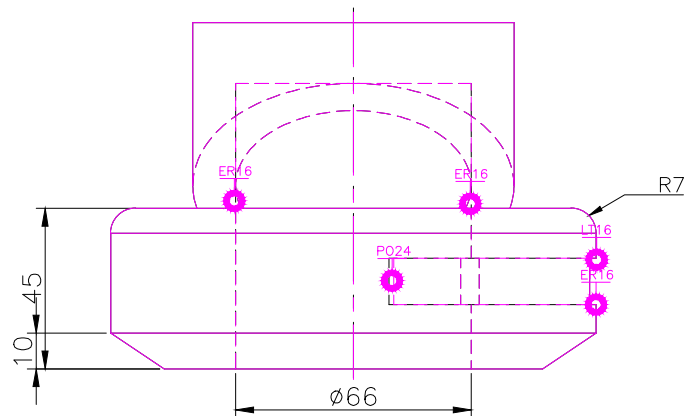
FRONT SCALE 1/2
