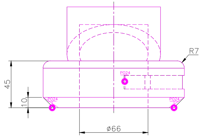
FRONT SCALE 1/2
