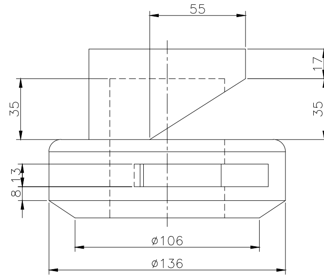
RIGHT SCALE 1/2
