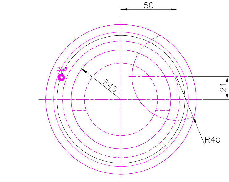
TOP SCALE 1/2
