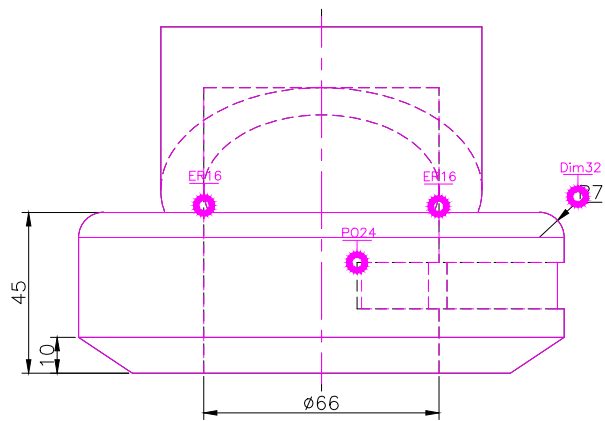
FRONT SCALE 1/2
