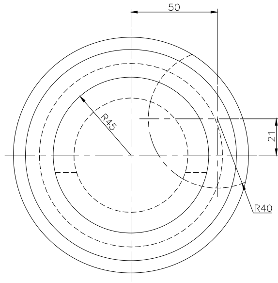
TOP SCALE 1/2
