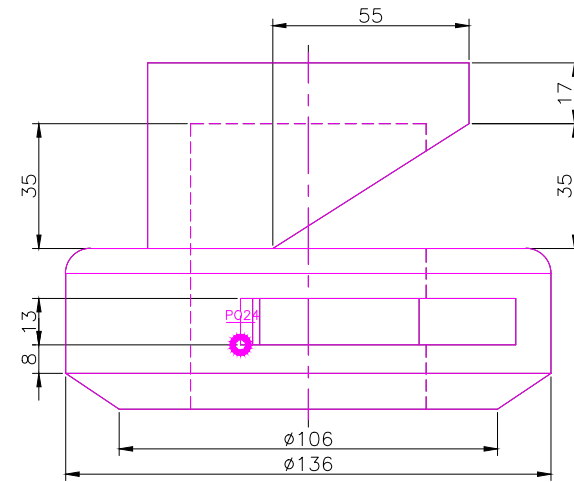
RIGHT SCALE 1/2
