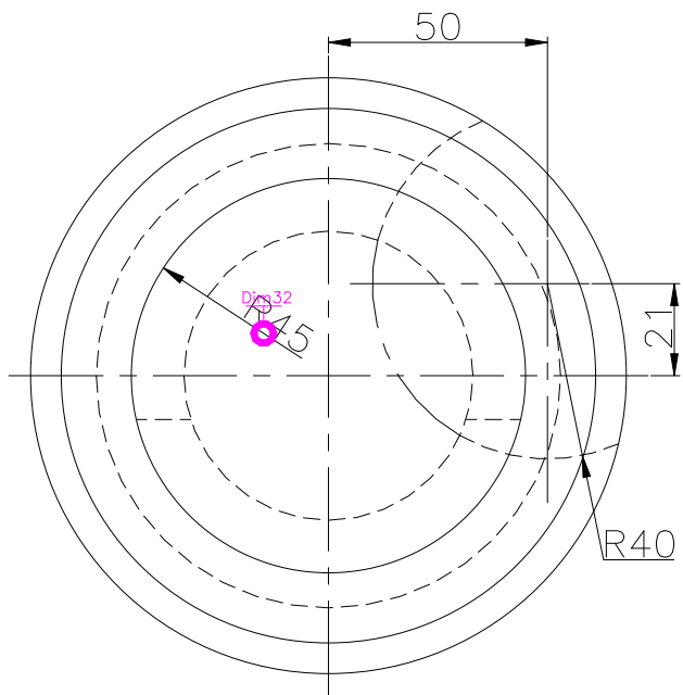
TOP SCALE 1/2
