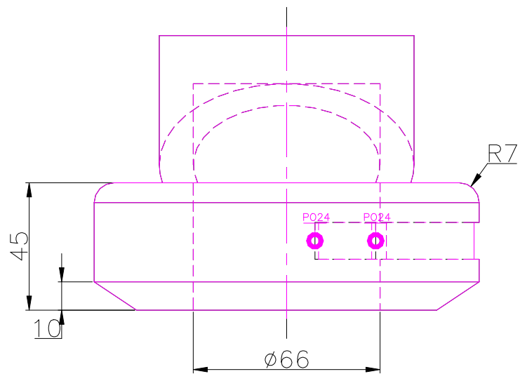
FRONT SCALE 1/2
