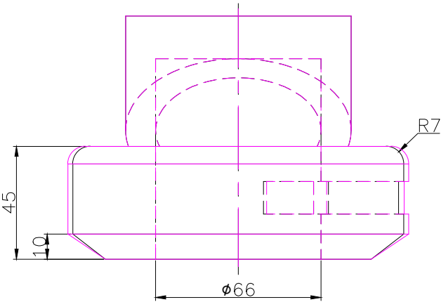
FRONT SCALE 1/2
