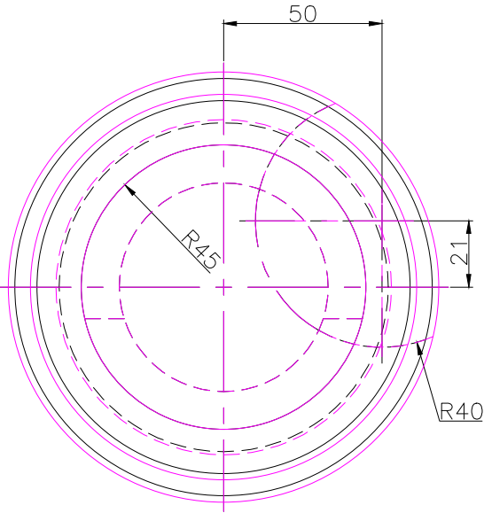
TOP SCALE 1/2
