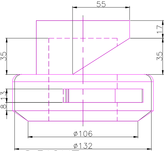
RIGHT SCALE 1/2
