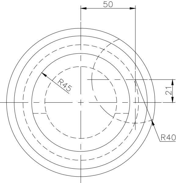
TOP SCALE 1/2
