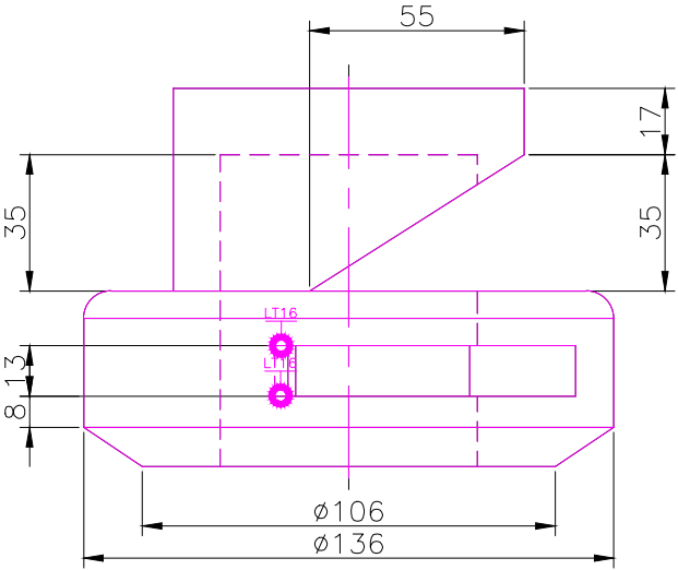
RIGHT SCALE 1/2
