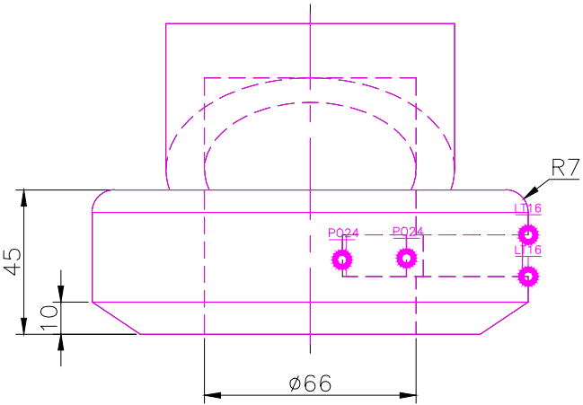
FRONT SCALE 1/2
