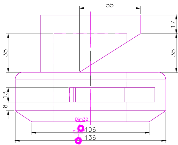
RIGHT SCALE 1/2
