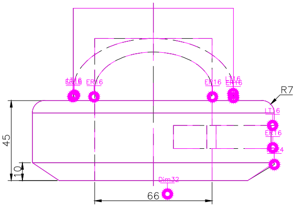
FRONT SCALE 1/2
