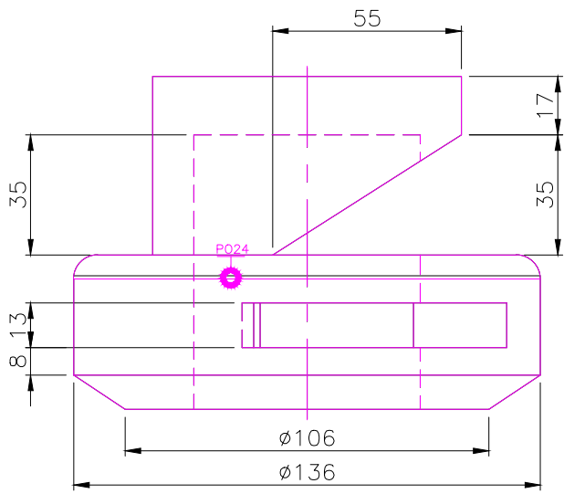
RIGHT SCALE 1/2
