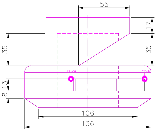
RIGHT SCALE 1/2
