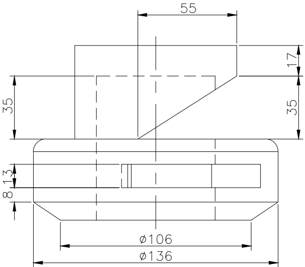
RIGHT SCALE 1/2
