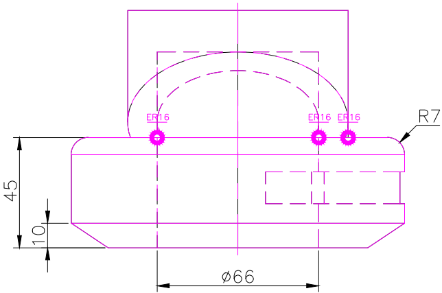
FRONT SCALE 1/2
