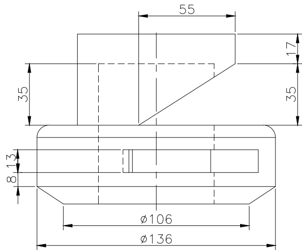
RIGHT SCALE 1/2
