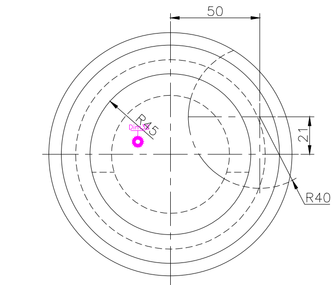
TOP SCALE 1/2
