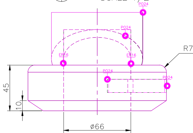
FRONT SCALE 1/2
