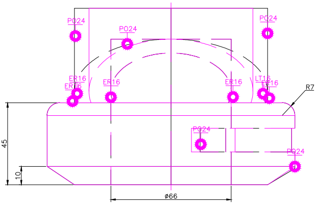
FRONT SCALE 1/2
