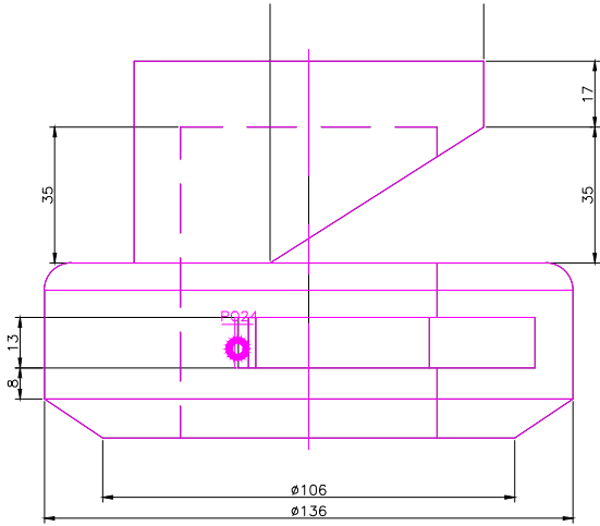
RIGHT SCALE 1/2
