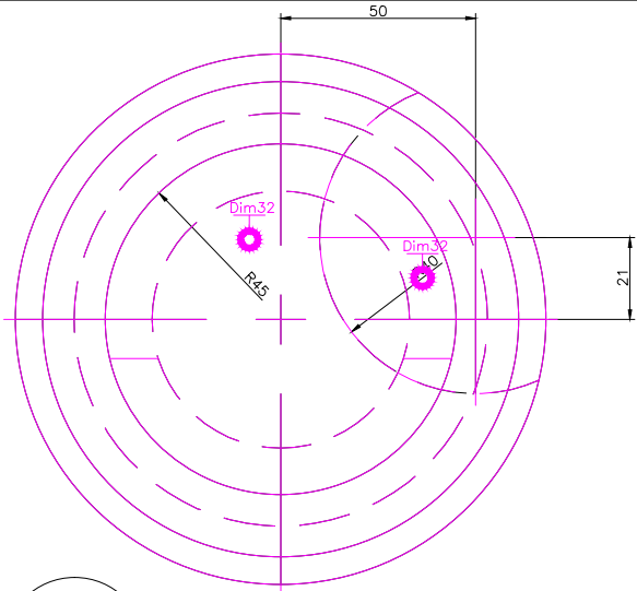
TOP SCALE 1/2
