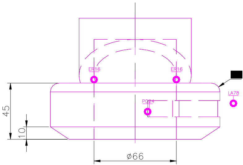
FRONT SCALE 1/2
