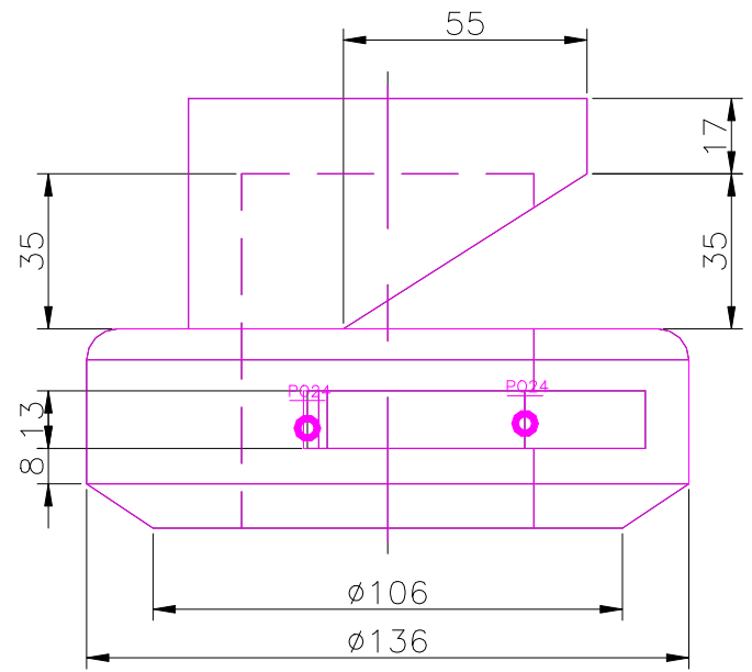
RIGHT SCALE 1/2
