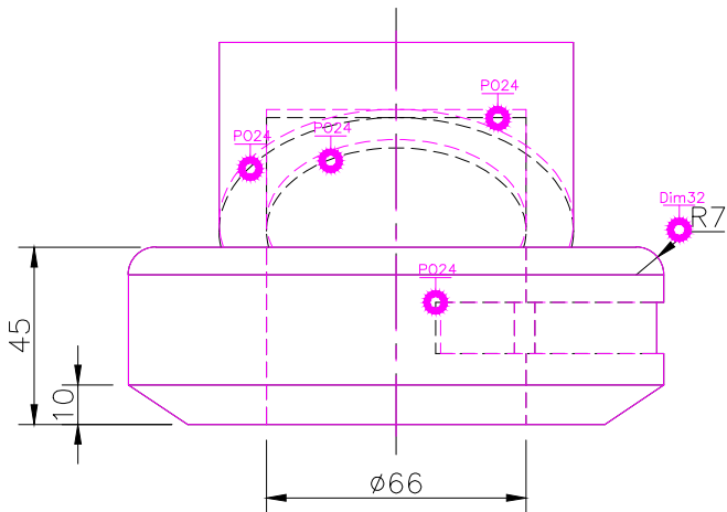
FRONT SCALE 1/2
