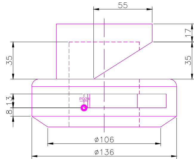
RIGHT SCALE 1/2
