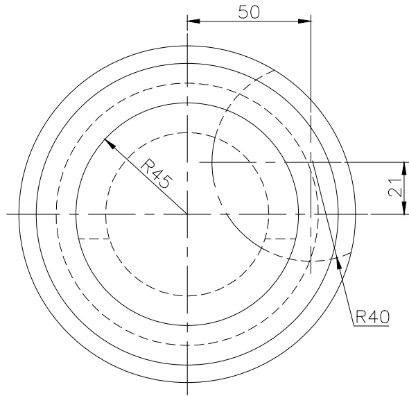
TOP SCALE 1/2
