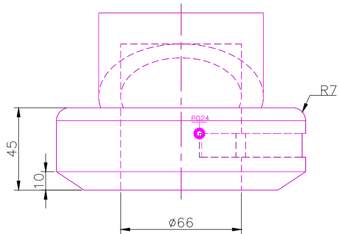
FRONT SCALE 1/2
