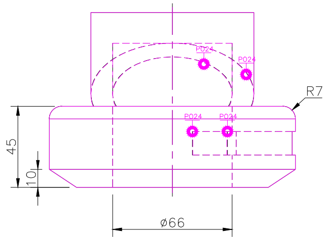
FRONT SCALE 1/2
