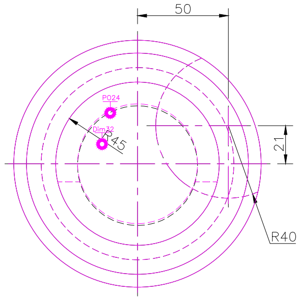
TOP SCALE 1/2
