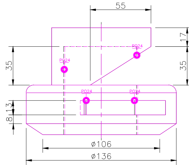
RIGHT SCALE 1/2
