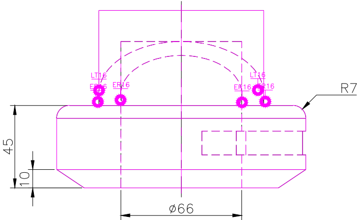
FRONT SCALE 1/2
