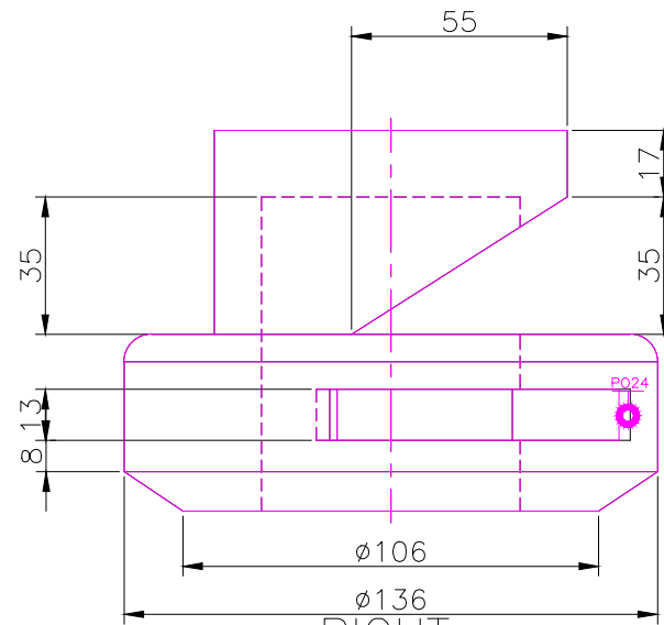
RIGHT SCALE 1/2
