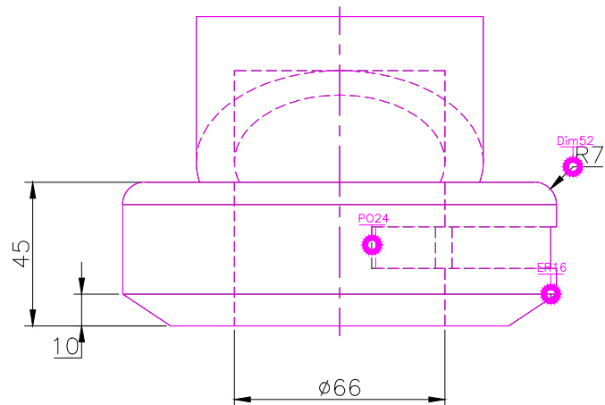
FRONT SCALE 1/2
