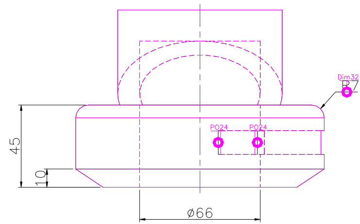
FRONT SCALE 1/2
