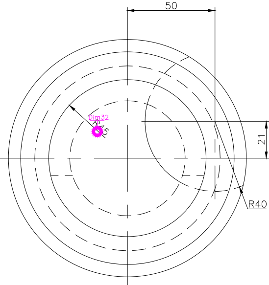
TOP SCALE 1/2
