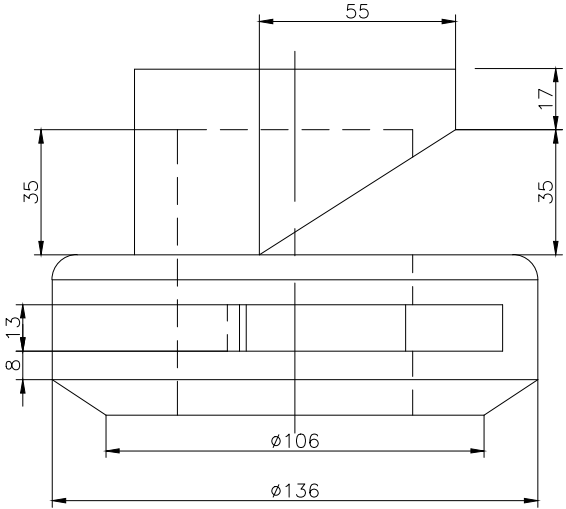
RIGHT SCALE 1/2
