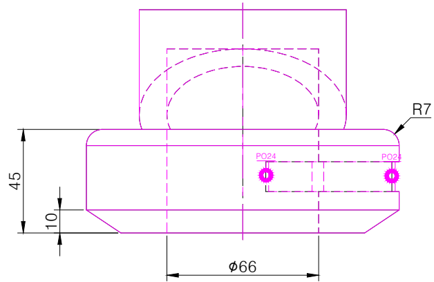
FRONT SCALE 1/2
