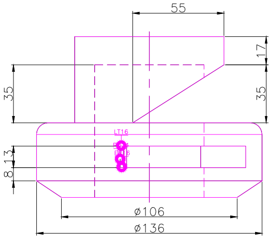
RIGHT SCALE 1/2
