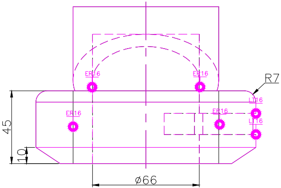
FRONT SCALE 1/2
