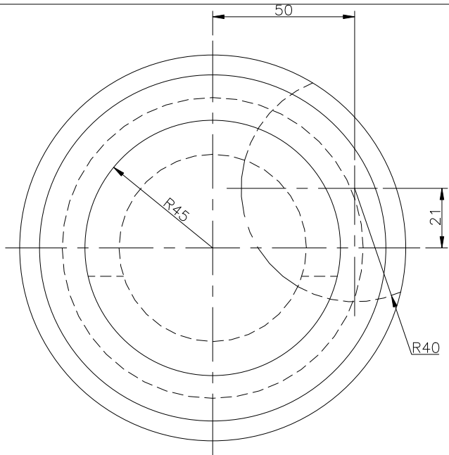
TOP SCALE 1/2
