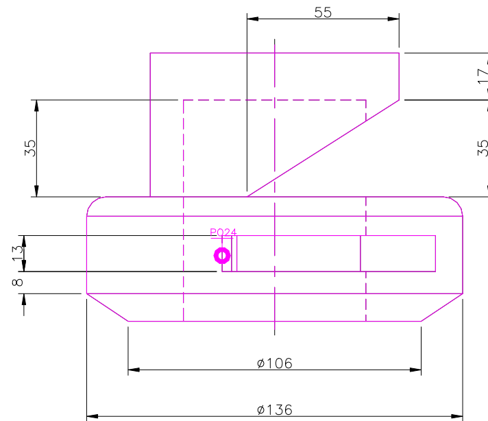
RIGHT SCALE 1/2
