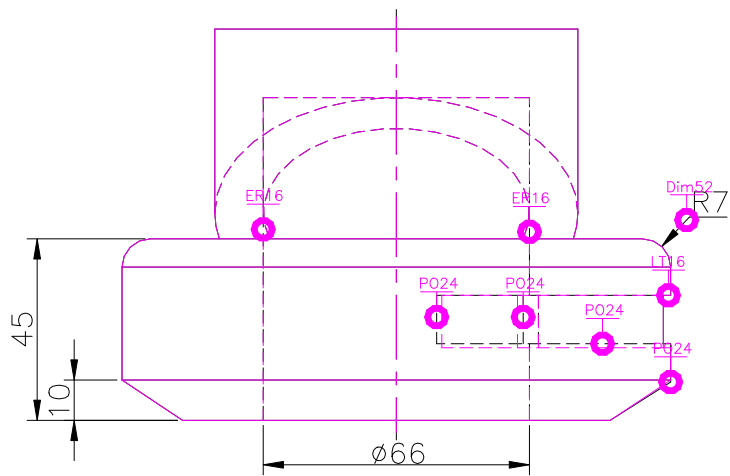
FRONT SCALE 1/2
