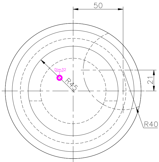
TOP SCALE 1/2
