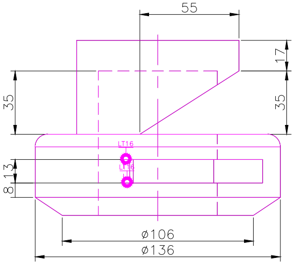
RIGHT SCALE 1/2
