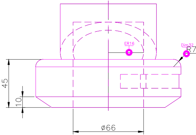
FRONT SCALE 1/2
