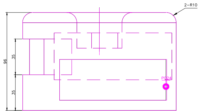
FRONT SCALE 1/2
