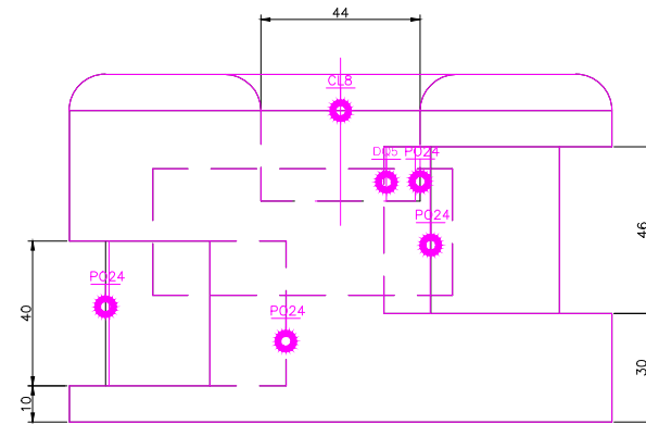
RIGHT SCALE 1/2
