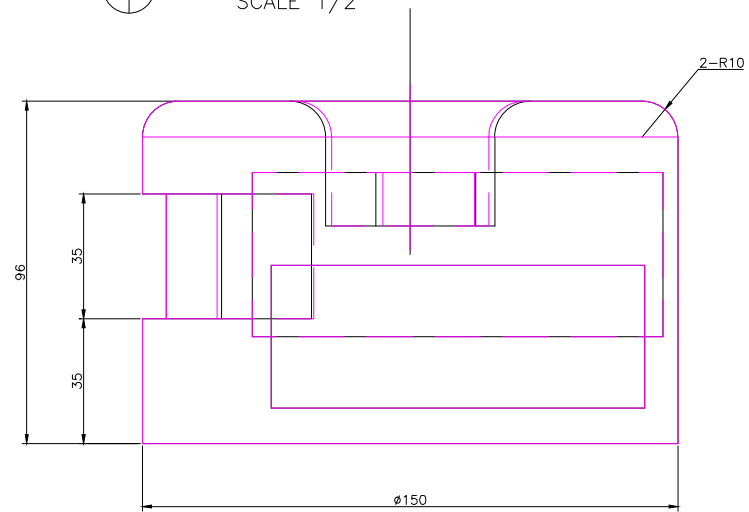
FRONT SCALE 1/2
