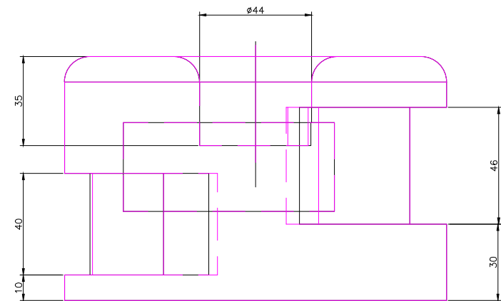
RIGHT SCALE 1/2
