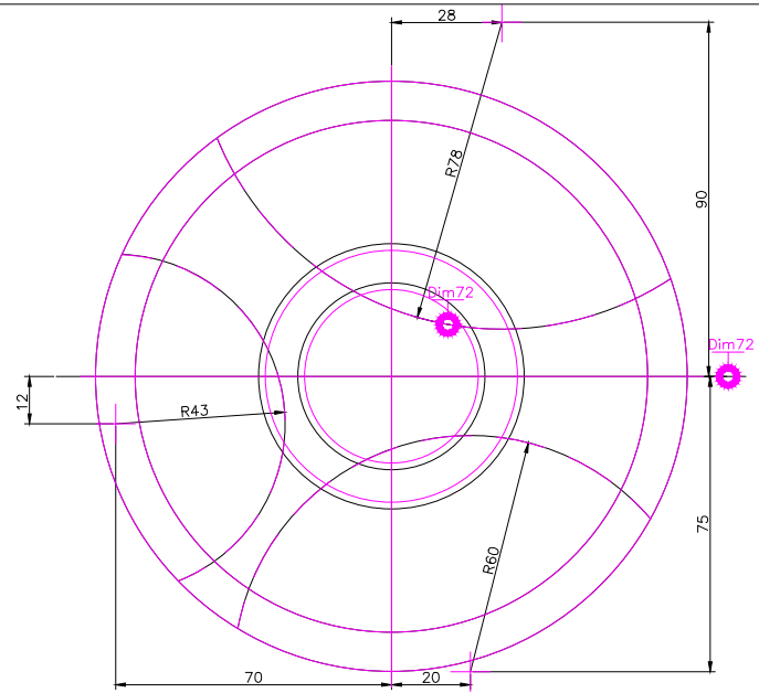
TOP SCALE 1/2
