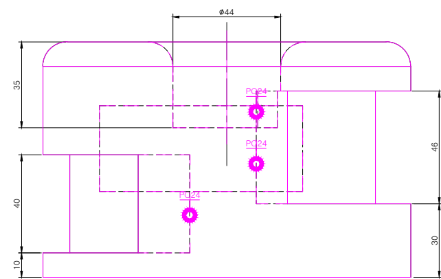
RIGHT SCALE 1/2
