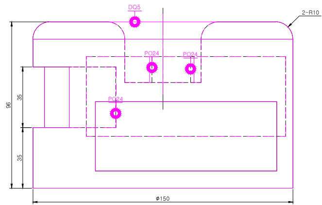
FRONT SCALE 1/2
