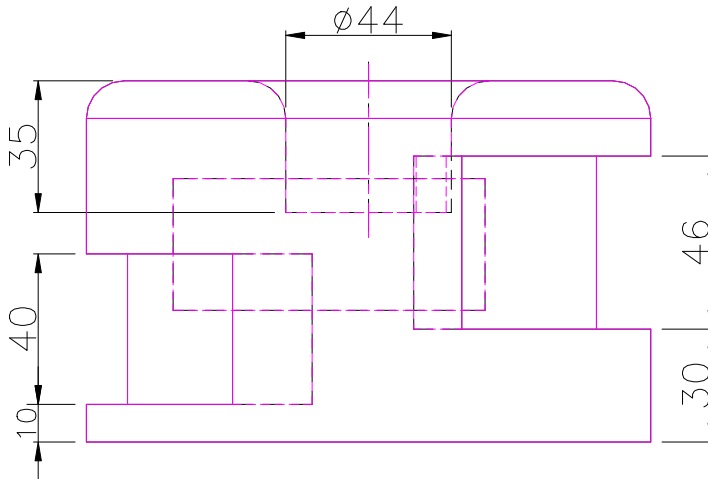
RIGHT SCALE 1/2
