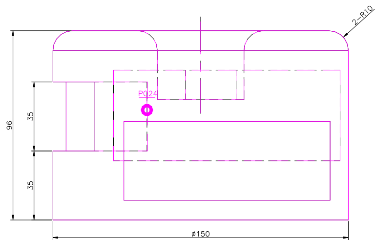
FRONT scale 1/2
