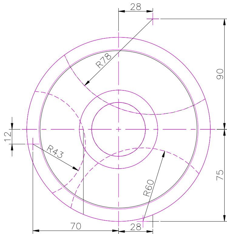
TOP SCALE 1/2
