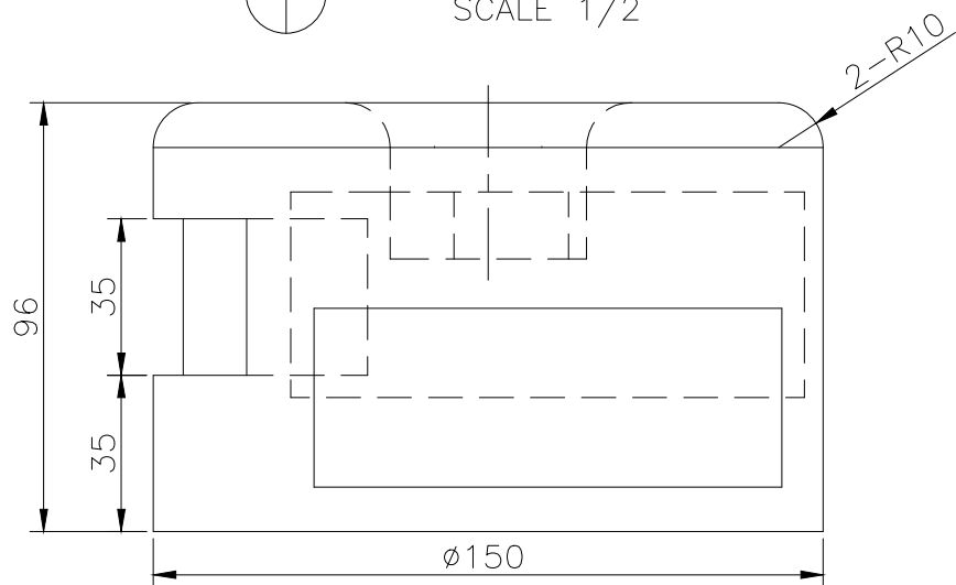
FRONT SCALE 1/2
