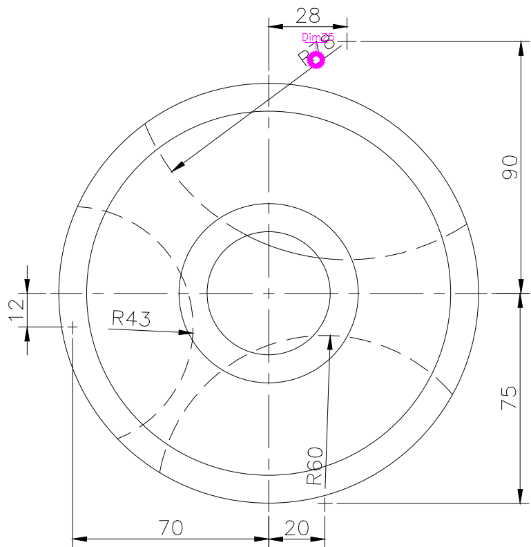
TOP SCALE 1/2
