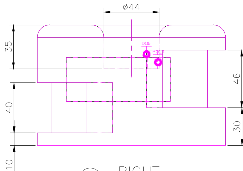
RIGHT SCALE 1/2
