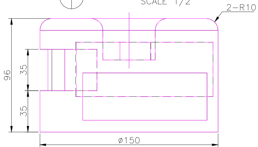
FRONT SCALE 1/2
