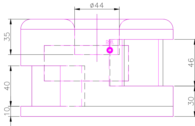
RIGHT SCALE 1/2
