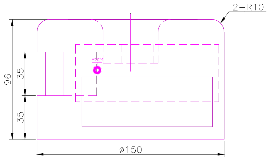
FRONT SCALE 1/2
