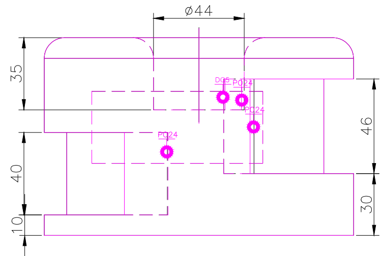
RIGHT SCALE 1/2
