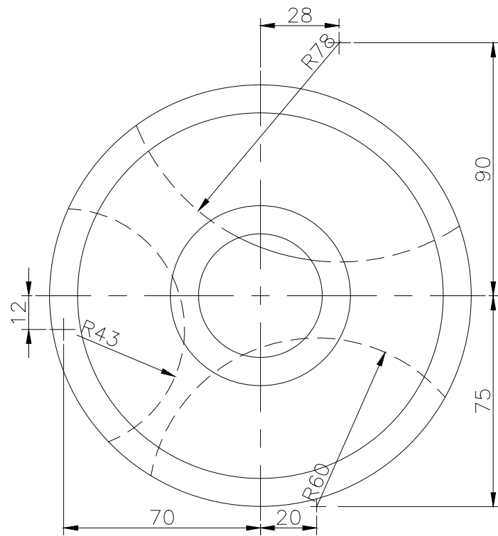
TOP SCALE 1/2
