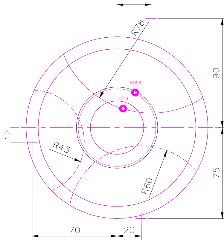
Top Scale 1/2
