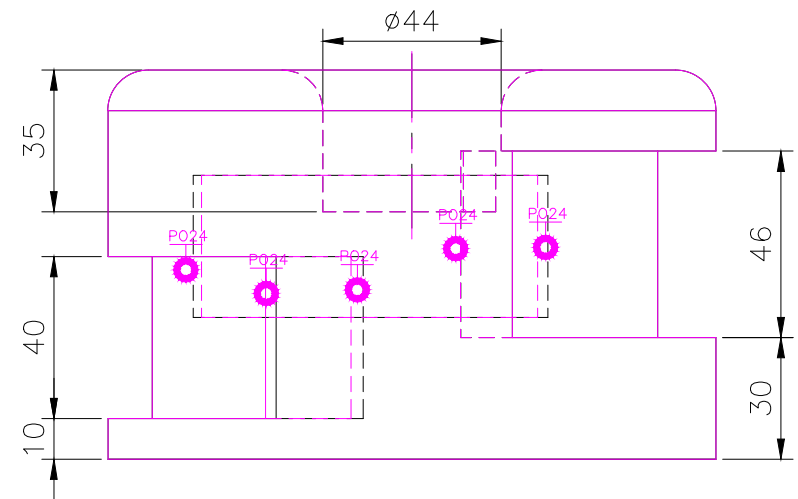
Right Scale 1/2
