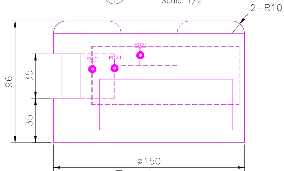
Front Scale 1/2
