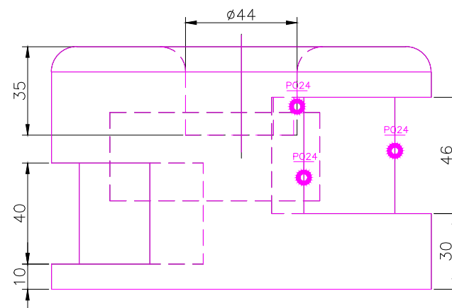
RIGHT SCALE 1/2
