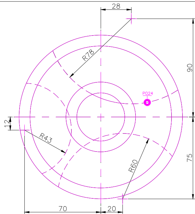
TOP SCALE 1/2
