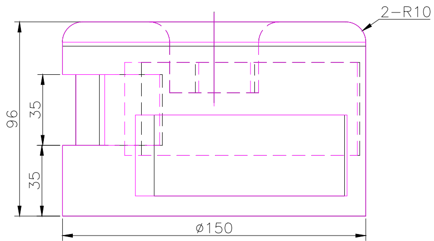
FRONT SCALE 1/2
