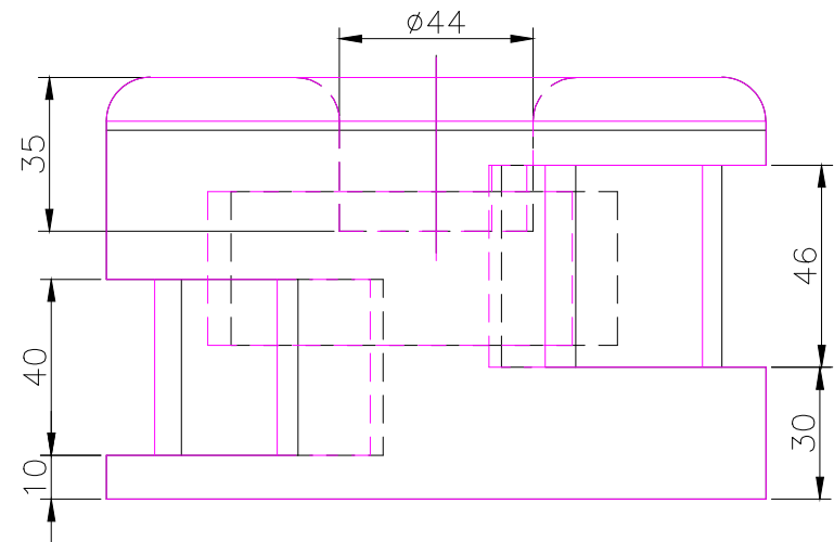
RIGHT SCALE 1/2
