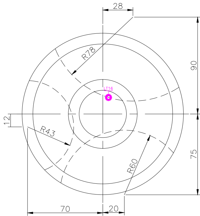
TOP SCALE 1/2
