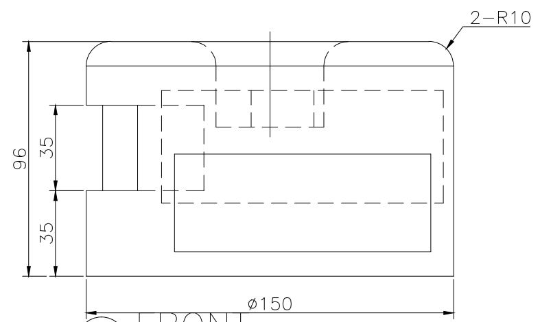
FRONT SCALE 1/2
