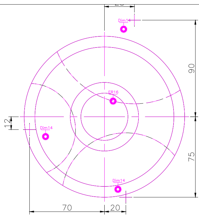
TOP SCALE 1/2
