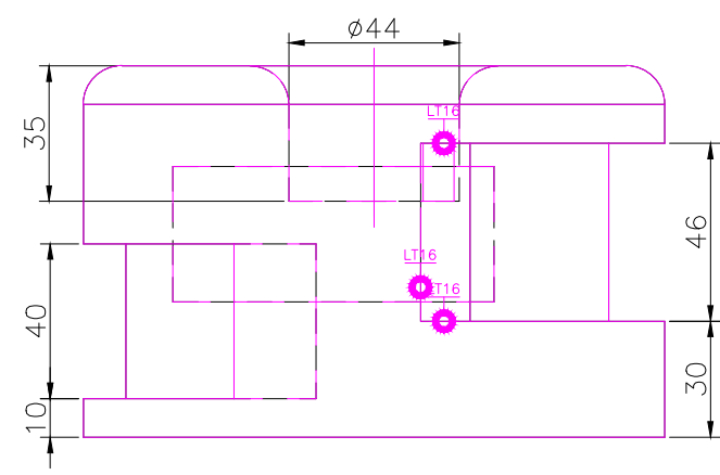
RIGHT SCALE 1/2
